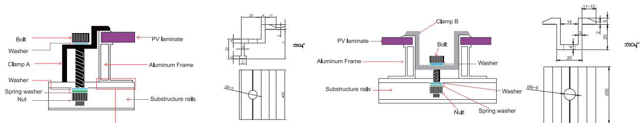
Figure 3 Clamp Details (Units:mm)
