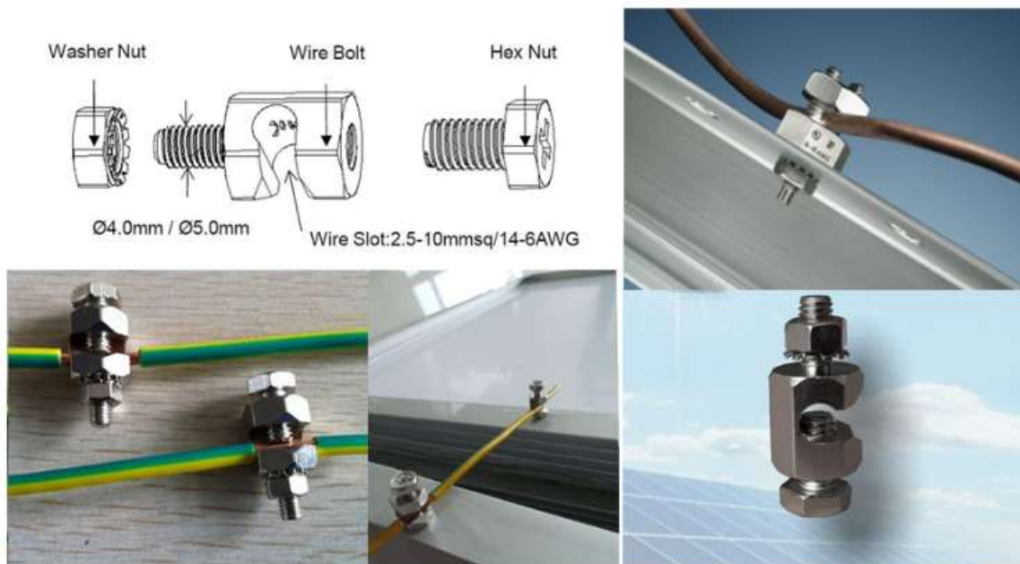
Figure 5: Installation methods
