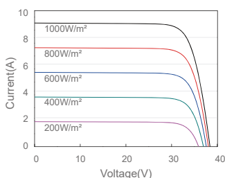
Current-Voltage Curve JAP60S01-270/SC/1000V
