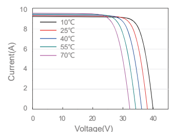
Current-Voltage Curve JAP60S01-270/SC/1000V
