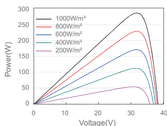
Power-Voltage Curve JAP60S01-270/SC/1000V
