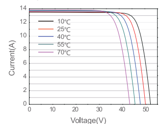
Current-Voltage Curve JAM72S30-540/MR/1500V
