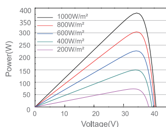
Power-Voltage Curve JAM60S21-380/MR/1000V
