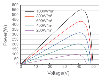
Power-Voltage Curve JAM72S30-555/GR/1500V
