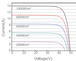
Current-Voltage Curve JAM72S30-555/GR/1500V
