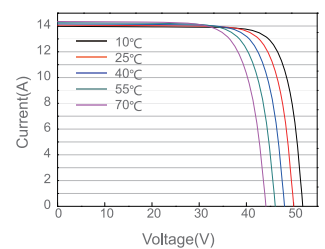
Current-Voltage Curve JAM72S30-555/GR/1500V
