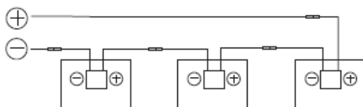
Series wiring
