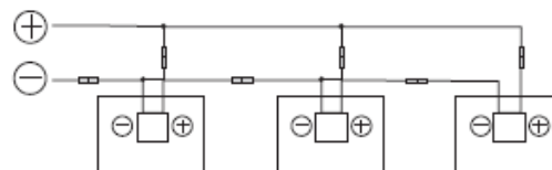
Parallel wiring
