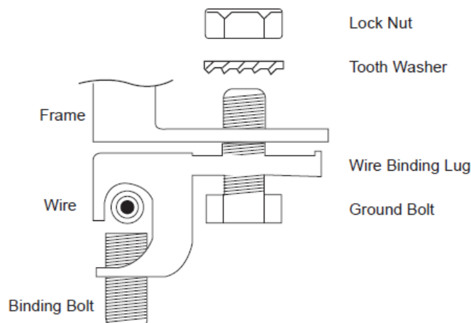
Figure 7: Installation Methods
