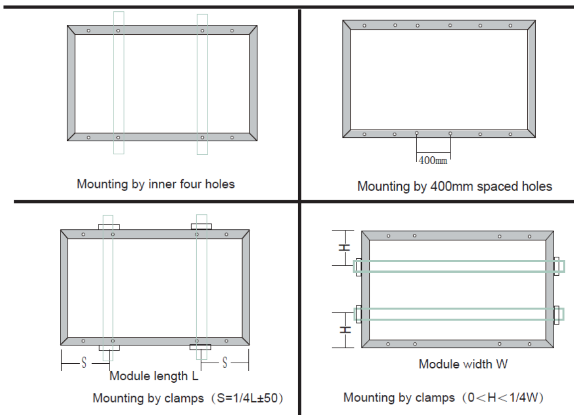
Figure 4 Installation methods
