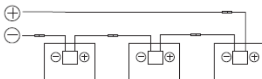
Series wiring
