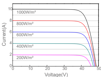
Current-Voltage Curve JAM72S01-380/PR/1000V
