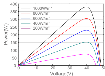
Power-Voltage Curve JAM72S01-380/PR/1000V
