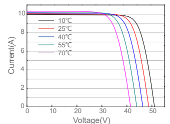
Current-Voltage Curve JAM72S01-380/PR/1000V
