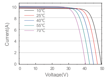
Current-Voltage Curve JAM72S01-355/PR/1000V
