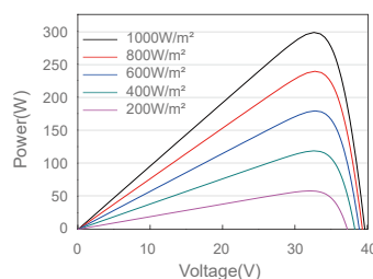
Power-Voltage Curve JAM60S02-300/PR/1000V
