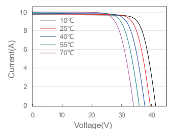
Current-Voltage Curve JAM60S02-300/PR/1000V
