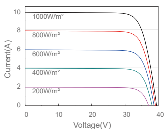
Current-Voltage Curve JAM60S02-300/PR/1000V
