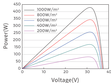
Power-Voltage Curve JAM54S31-430/LR/1500V
