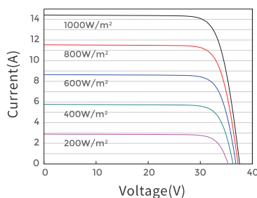
Current-Voltage Curve JAM54S31-430/LR/1500V
