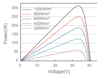
Power-Voltage Curve JAM60D00-310/BP
