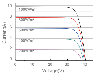
Current-Voltage Curve JAM60D00-310/BP
