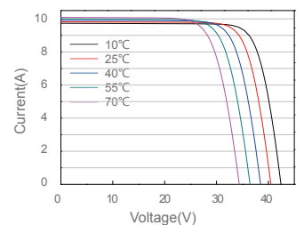
Current-Voltage Curve JAM60D00-310/BP
